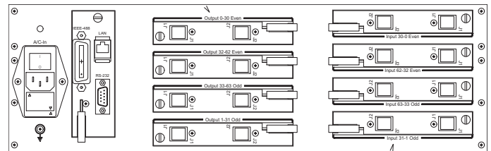
DXM/64x64 Mainframe Chassis
