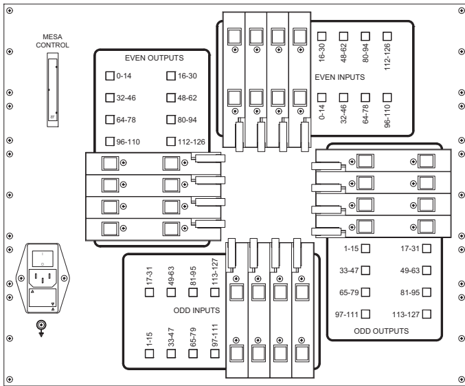
DXM/128x128 Expansion Chassis with Densi-Shield Signal Connections
